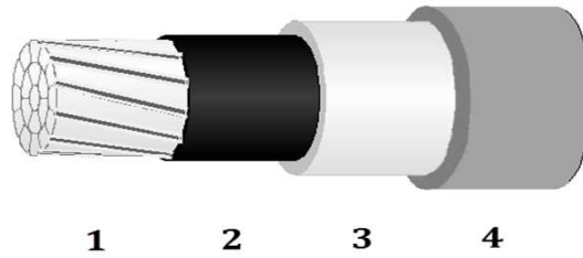
69 kV AERIAL CABLE 795 KCM AAC (403mm 2 ) 75° C GRAY
